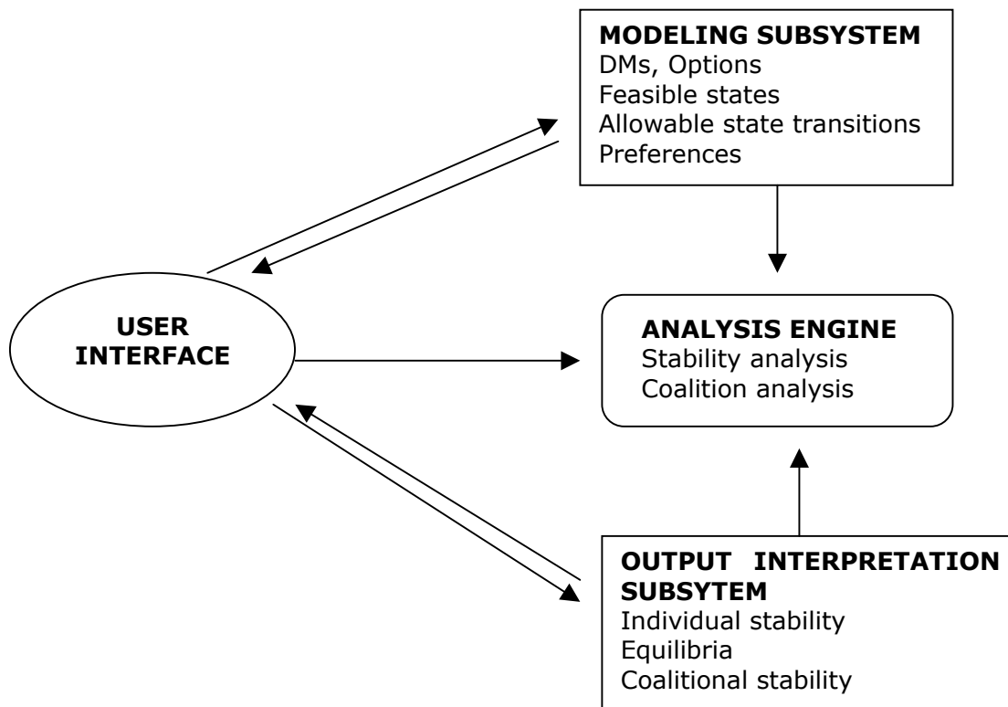
Figure 4.6. GMCR II structure
