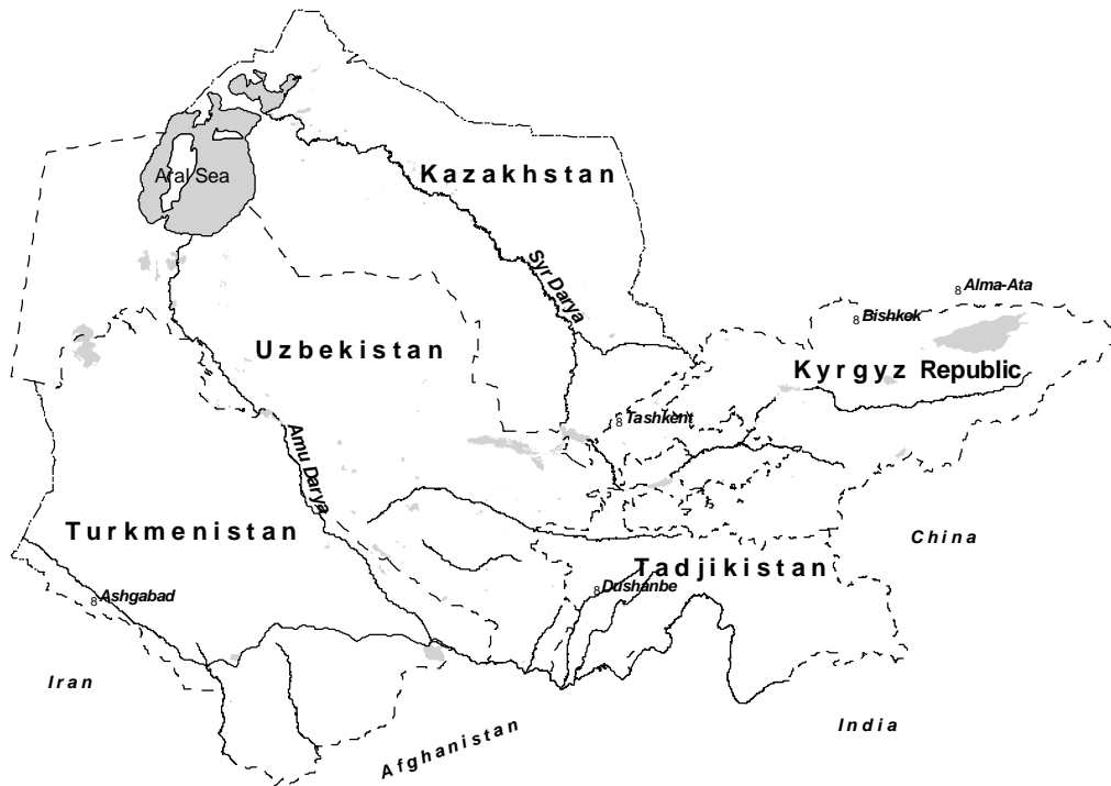
Figure 4.15. The Aral Sea basin
