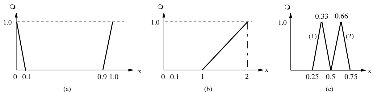
Figure 5.3. Fuzzy input for the Tisza River problem
