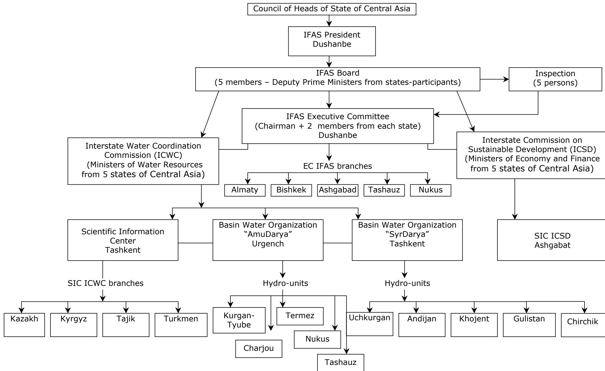
Figure 4.16. Structure of International Fund of Aral Sea Saving (IFAS)
