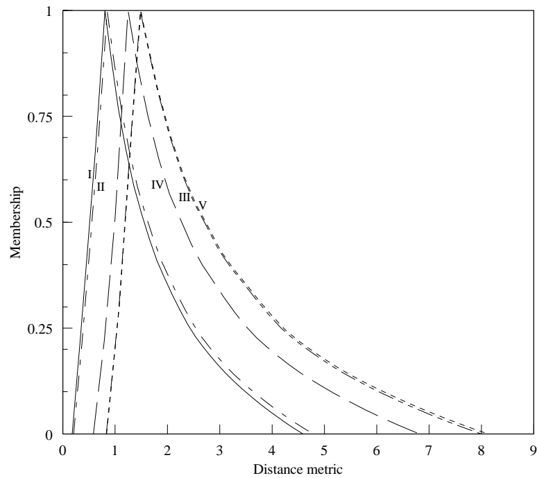
Figure 5.4. Distance metrics for the Tisza River problem
