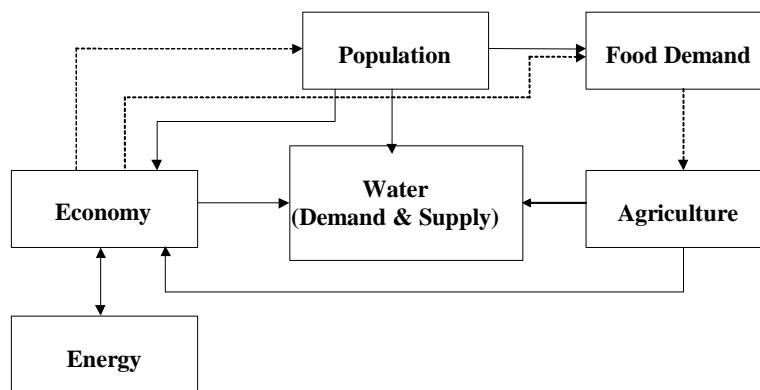
Figure 4.20. Structure of the Aral Sea basin sustainable development model
