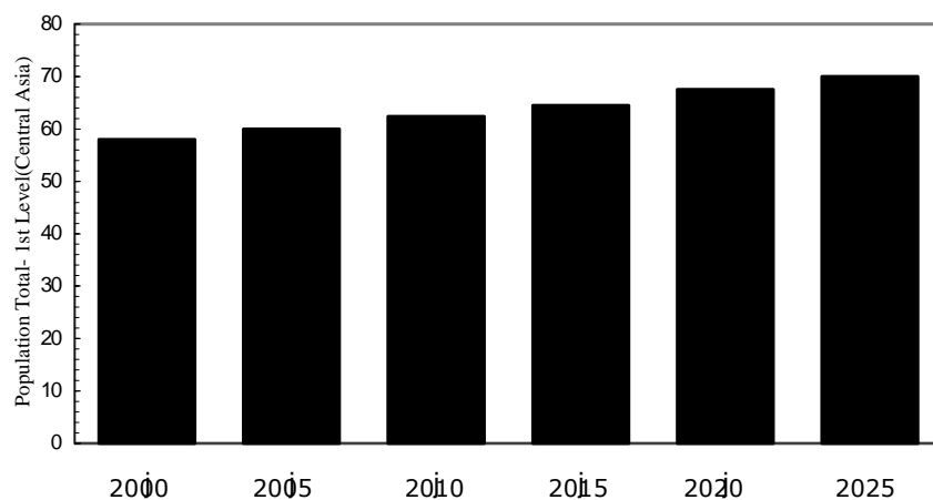
Figure 4.17. Population Projections (UN Low)
