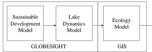
Figure 4.19. Aralmod block diagram
