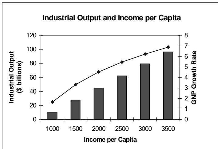
Figure 4.18 Industrial output necessary to reach various levels of income per capita
