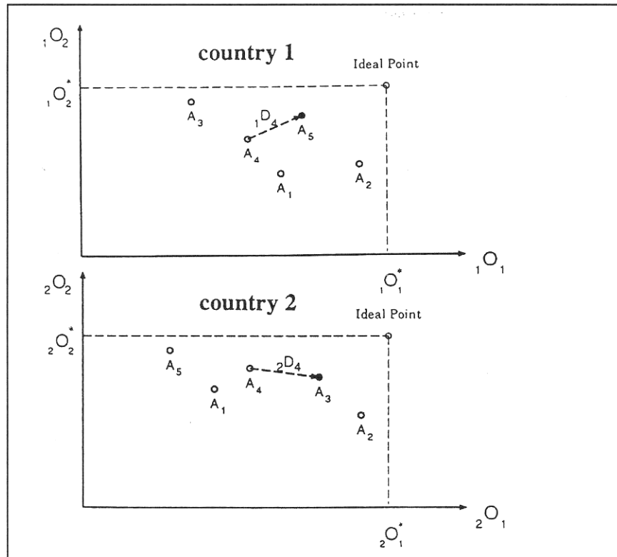
Figure 4.5. Schematic representation of the performance of the alternatives within a bi-objective framework for both countries
